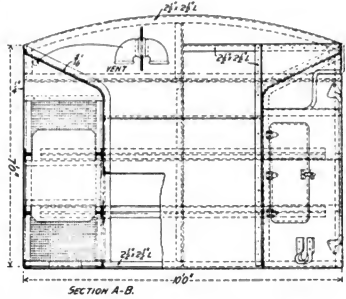
Fig. 4067. Cross-Section of 7,000-Gallon Tender Tank. Louisville & Nashville.
